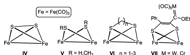
Chart 3. “Open” and “Closed” Fe 2 S 2 Cluster Types
