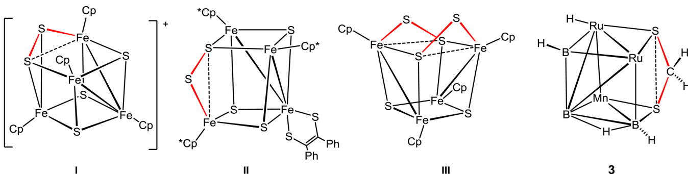
Chart 2. Cubane-Type Clusters with Bridging Atom between Two Vertices a
